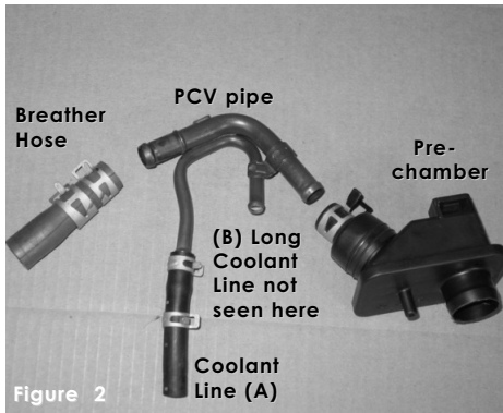
Figure 2 The assembled PCV pipe, hose and vent chamber are disassembled to be used separately. The only parts used are the Breather hose, vent chamber and the long coolant (B) not seen in the picture.
