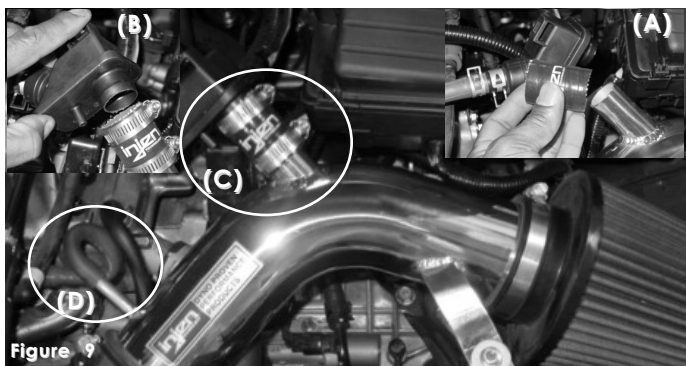
Figure 9 Press the 1 1/8" x 2" hose over the large port on the intake, use the two mini clamps in this kit to secure the hose(A). Press the assembled vent chamber port into the large hose on the intake(B). This illustration shows a filter on the end of the intake to be used as a short ram.
