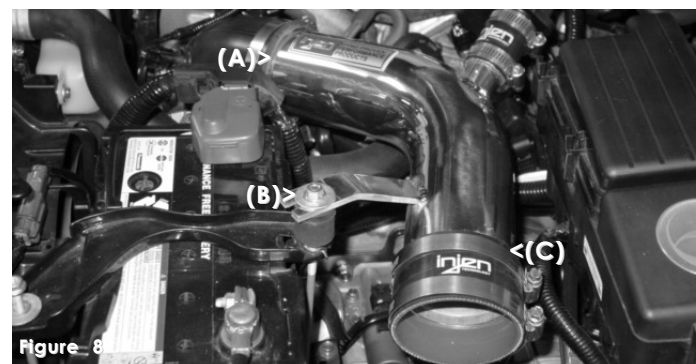
Figure 8 Press the primary intake into the elbow on the throttle body(A) and line up the bracket on the intake to the vibra-mount stud(B), use the m6 nut and washer to hold the intake in place. The 3" hose on the end of the intake is only used on the RD1680 for the secondary intake (C).
