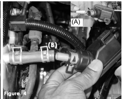
Figure 4 Press the 1 1/2" x 1/2" aluminum coupler into the vent chamber (A) and connect to breather line(B). Press the coupler into the chamber then into the stock breather hose on the crankcase(B).
