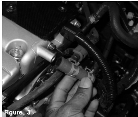
Figure 3 Remove the breather hose from the PCV pipe and press it over the crankcase port. Use the stock hose clamps to secure the lines in place.
