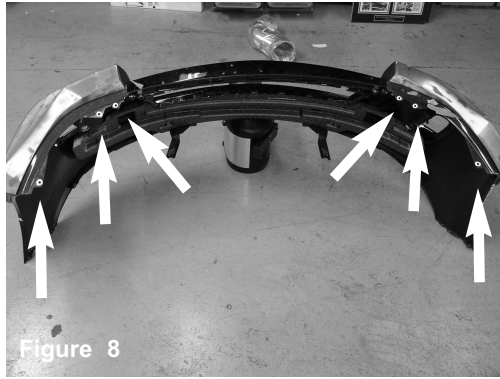
Figure 8 Bumper shown removed from vehicle showing 6 additional clips that will need to be removed from the bottom.
