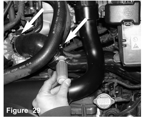
Figure 29 With the pipe in place, make your final adjustments for the best fitment and then tighten both clamps on the 90 deg. elbow located on the throttlebody.
