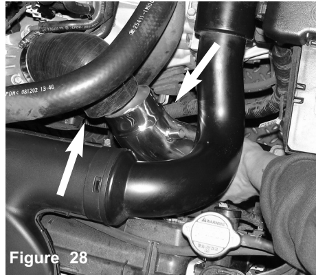
Figure 28 Slide the intake pipe from the bottom and work the pipe into the 90 deg. hose already located on the throttlebody.
